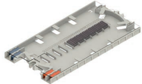
COYOTE LITE-GRIP Long Deep Profile Splice Tray Kit for Ribbon/Mass Fusion Splices (216 Splice CT.)
