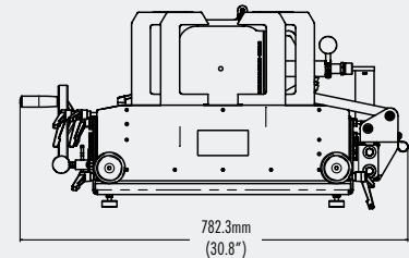
SMARTFAB 125 with Heater Extended
