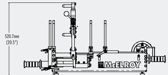
SMARTFAB 125 with Heater Extended
